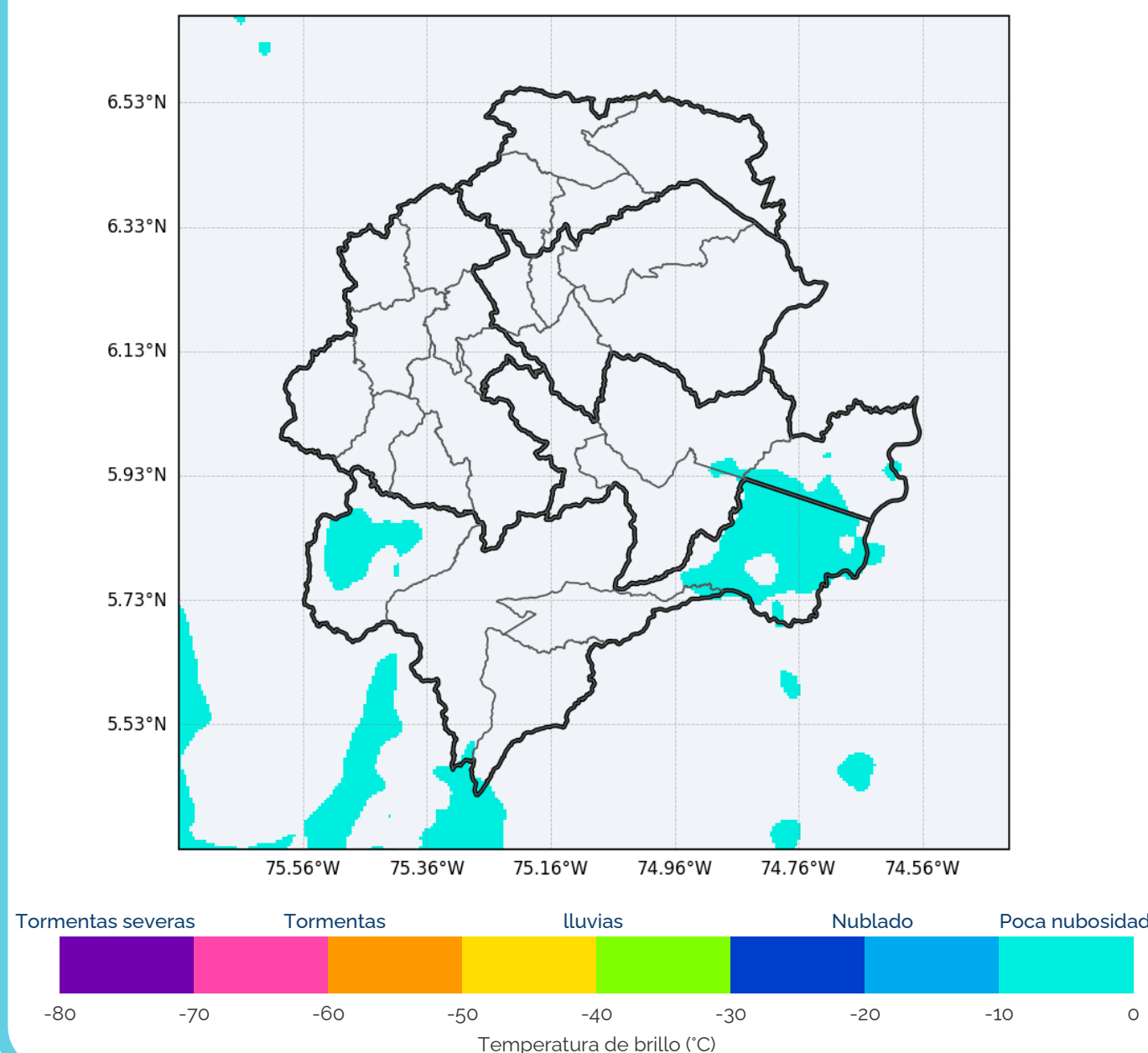
OLR Canal 13 GOES-19 + GLM 30/06/2026 08:10
