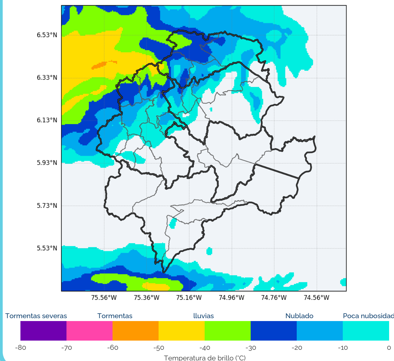
OLR Canal 13 GOES-19 + GLM 26/06/2026 07:50
