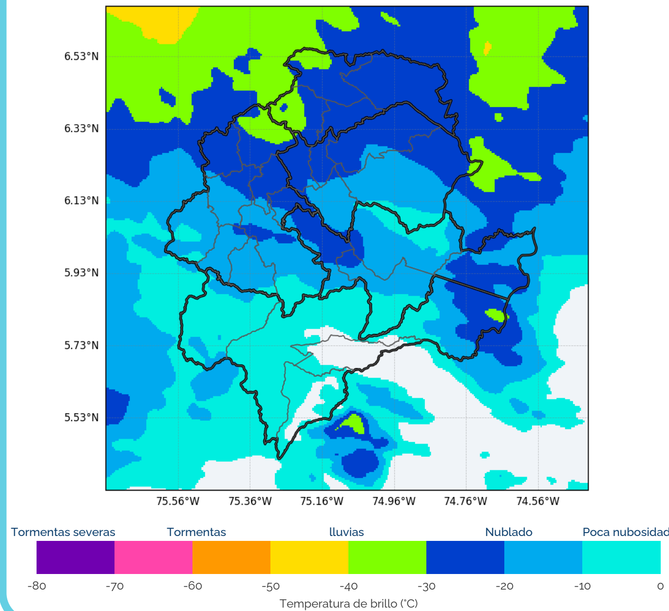
OLR Canal 13 GOES-19 + GLM 25/06/2026 08:10
