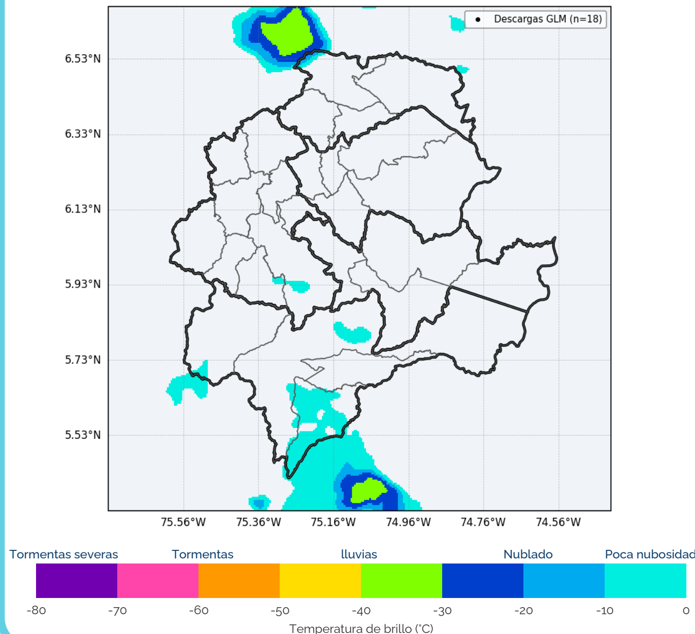
OLR Canal 13 GOES-19 + GLM 29/07/2026 07:50
