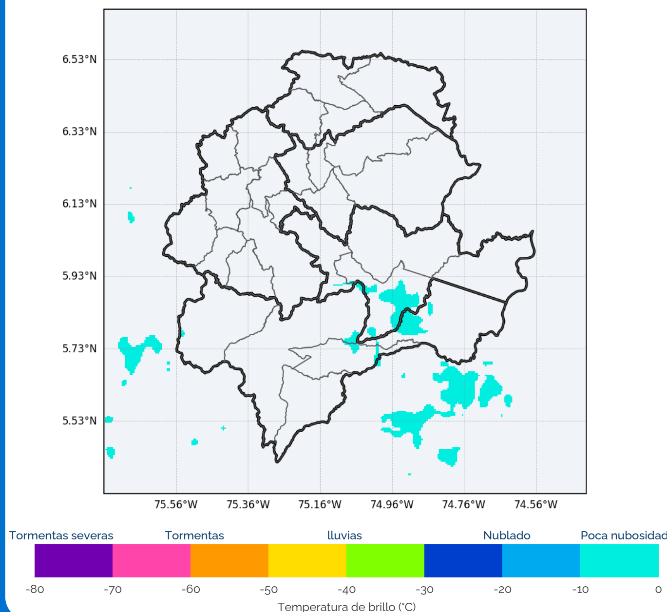
OLR Canal 13 GOES-19 + GLM 24/07/2026 17:20
