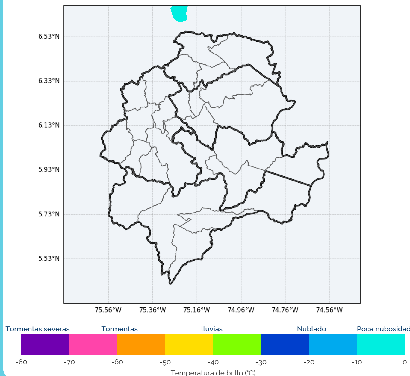
OLR Canal 13 GOES-19 + GLM 22/07/2026 08:10
