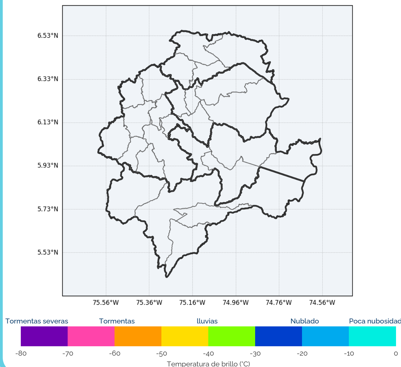
OLR Canal 13 GOES-19 + GLM 14/07/2026 08:10
