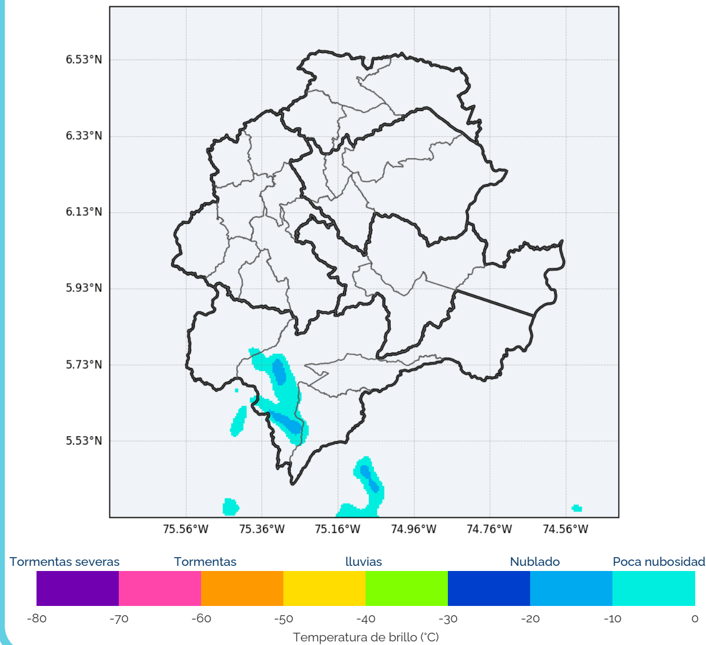
OLR Canal 13 GOES-19 + GLM 10/07/2026 08:10
