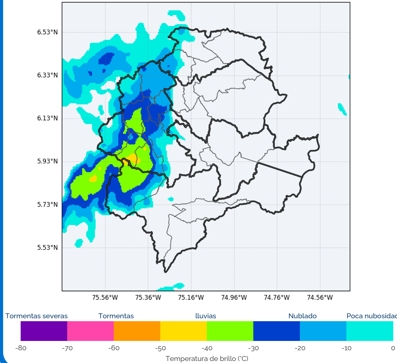
OLR Canal 13 GOES-19 + GLM 07/07/2026 17:20
