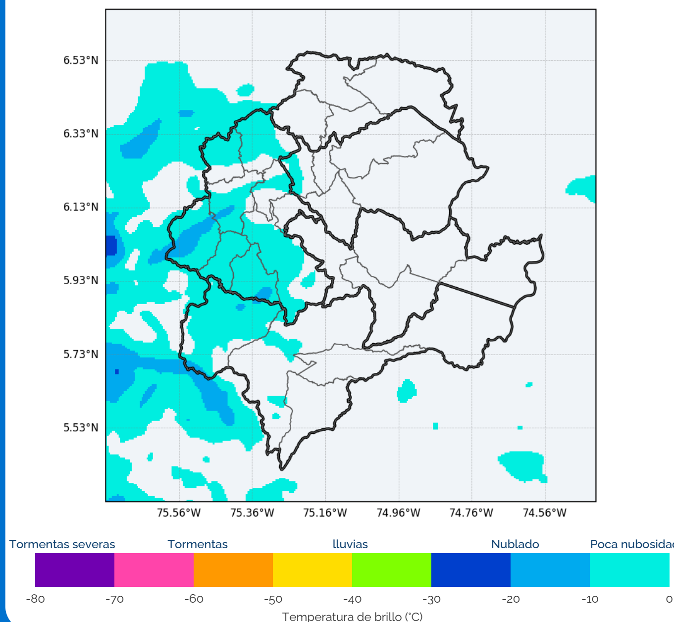
OLR Canal 13 GOES-19 + GLM 12/08/2026 17:20
