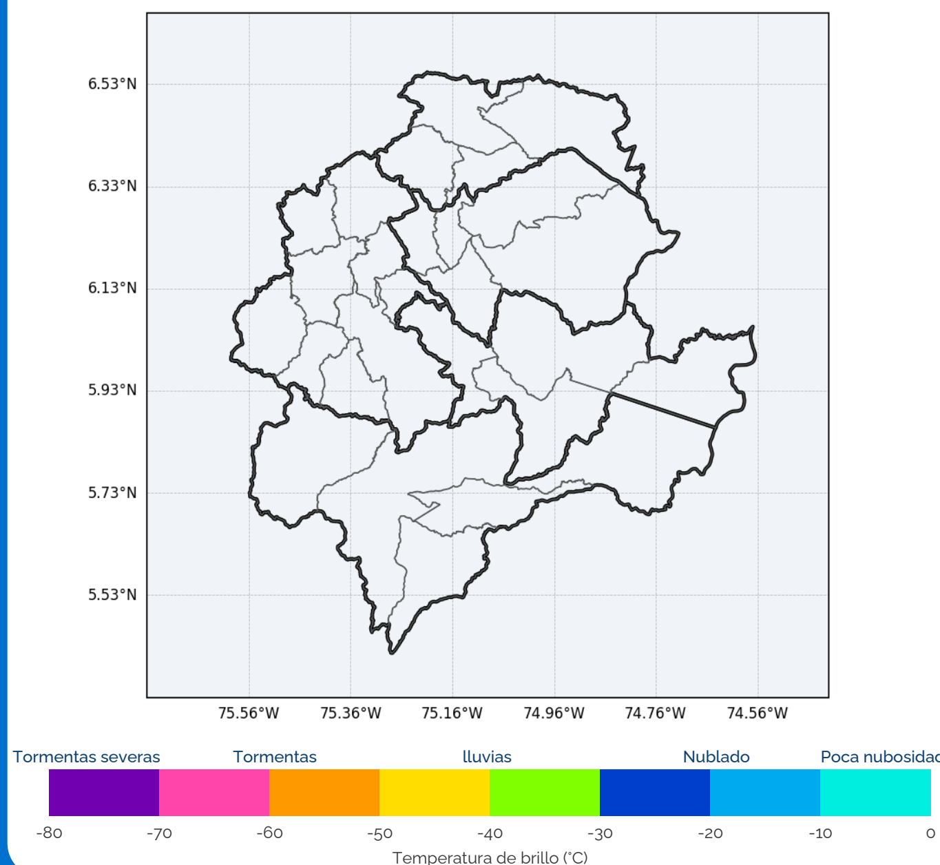
OLR Canal 13 GOES-19 + GLM 10/08/2026 17:20
