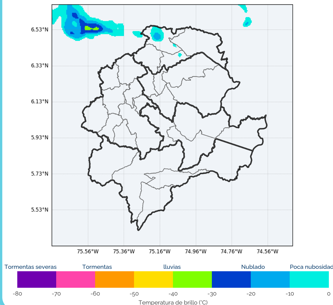
OLR Canal 13 GOES-19 + GLM 10/08/2026 08:10
