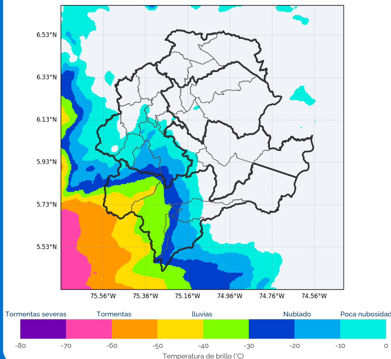
OLR Canal 13 GOES-19 + GLM 25/08/2026 17:20
