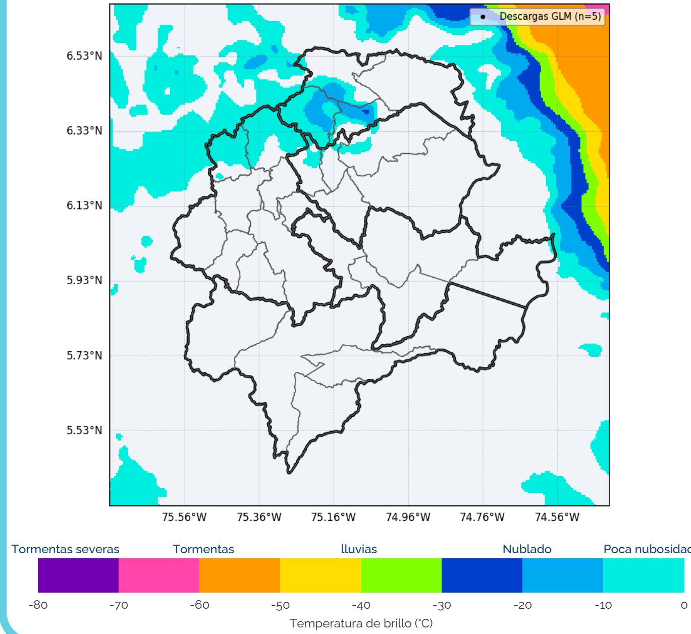
OLR Canal 13 GOES-19 + GLM 21/08/2026 08:10
