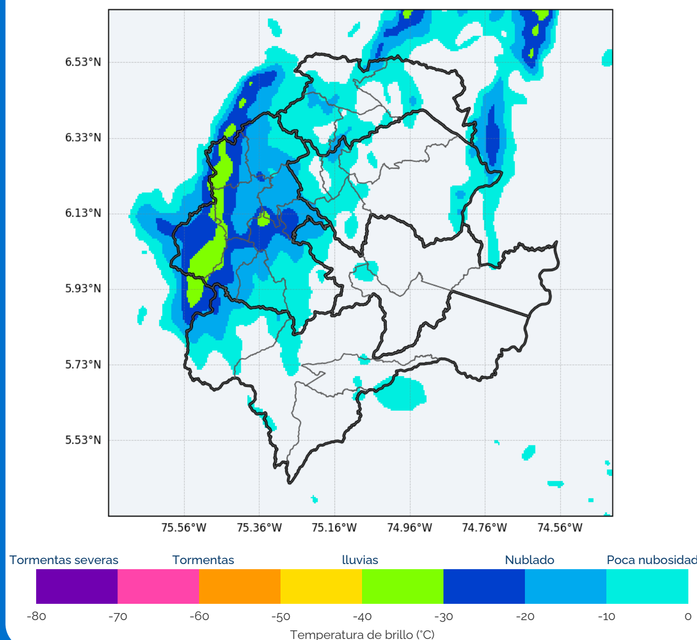
OLR Canal 13 GOES-19 + GLM 20/08/2026 17:20
